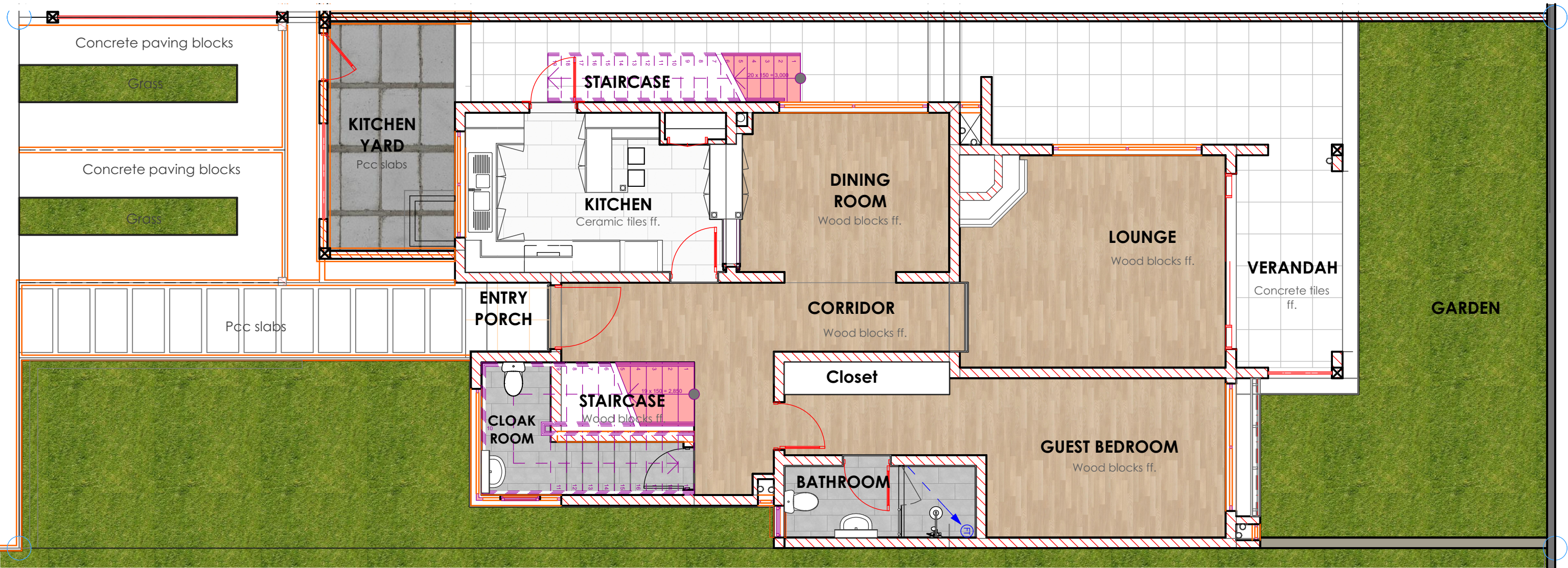
Ground Floor Plan = 116.65m 2
