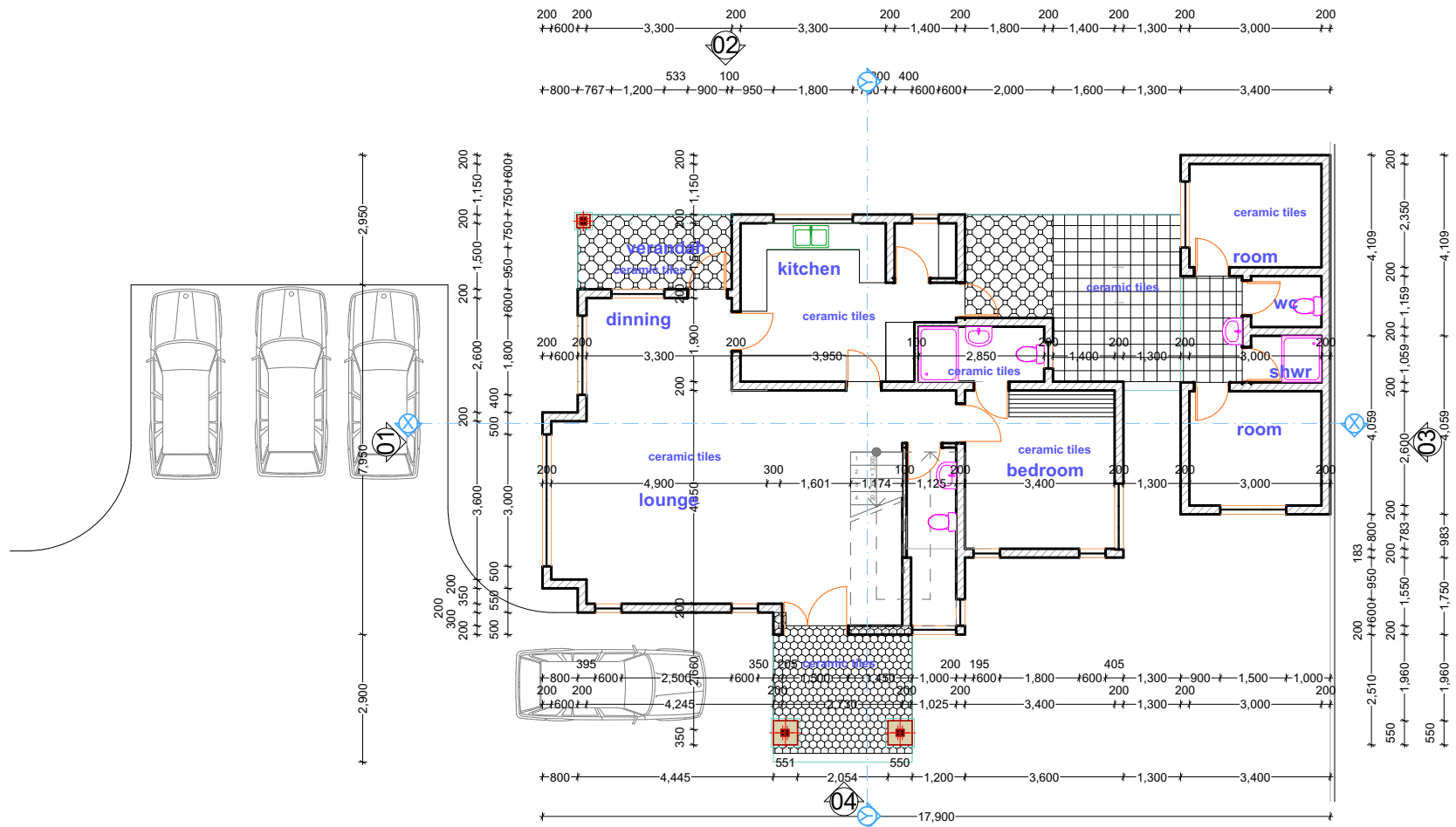
GROUND FLOOR PLAN - TYPE A
